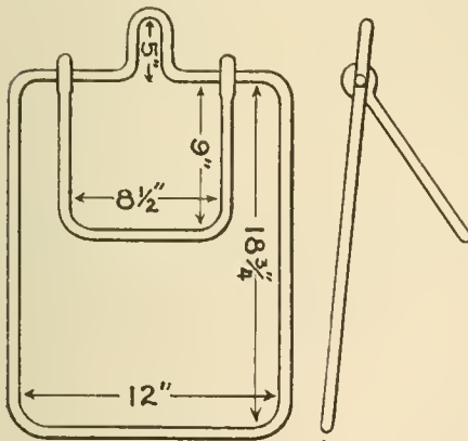
HANDY AIR PUMP LIFTER.
